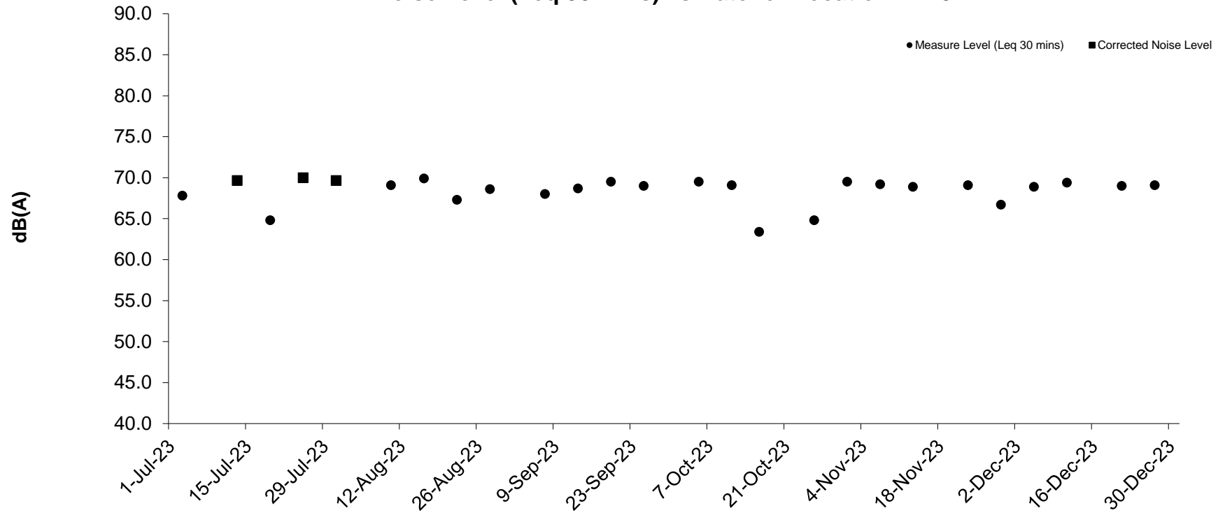
Noise Level (Leq 30 mins) vs Date for Location M-N3
